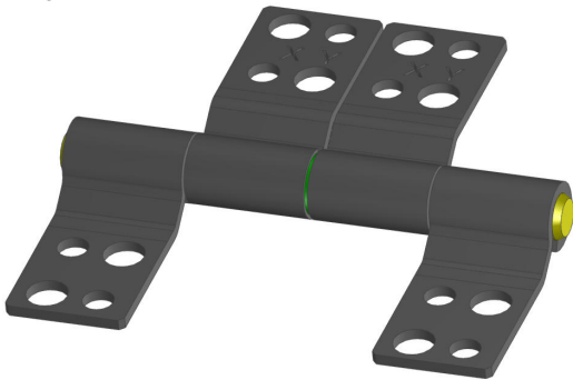
SB 188 Life Test 80,000 Cycles
