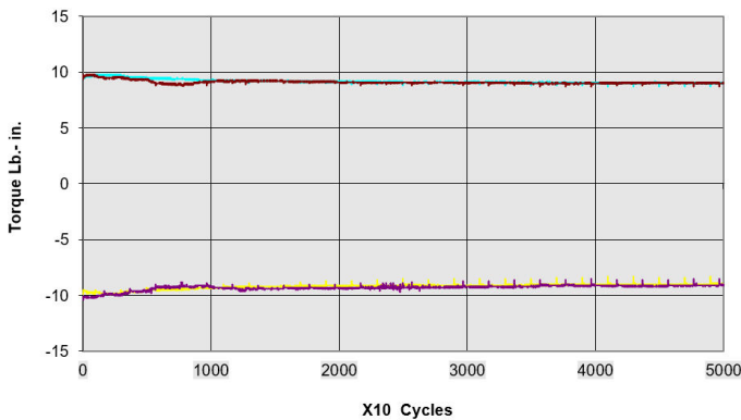
ZC 188 Life Test 50,000 Cycles
