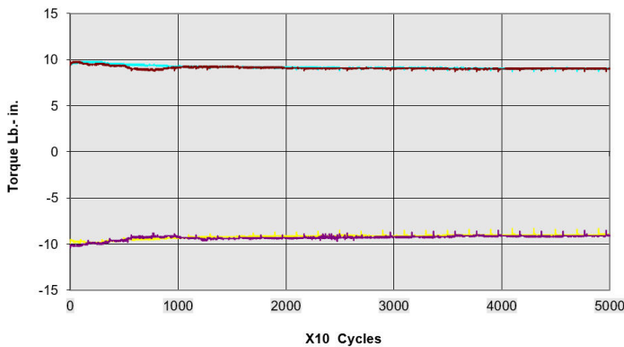
ZC 188 Life Test 50,000 Cycles
