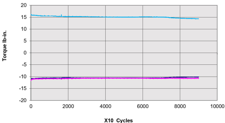
SB 200 Life Test 90,000 Cycles
