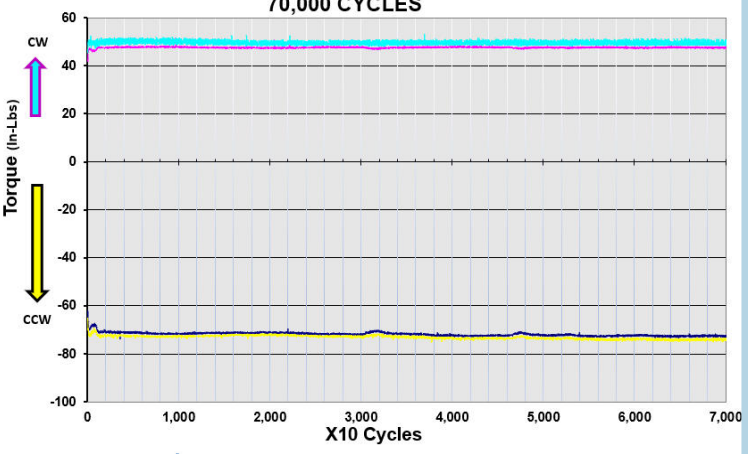
SB 500 SB 101 LIFE TEST 70,000 CYCLES
