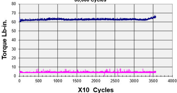
One Way Clutch 35,000 Cycles
